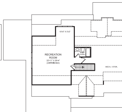
THIRD FLOOR
